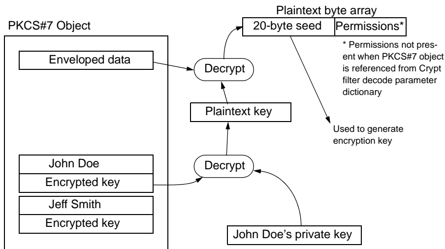
Figure 4 – Public-key encryption algorithm
